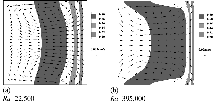
Figure 4. Temperature and velocity fields computed using the proposed surface layer model. Top plane ( y=0.9 ), steady flow.
