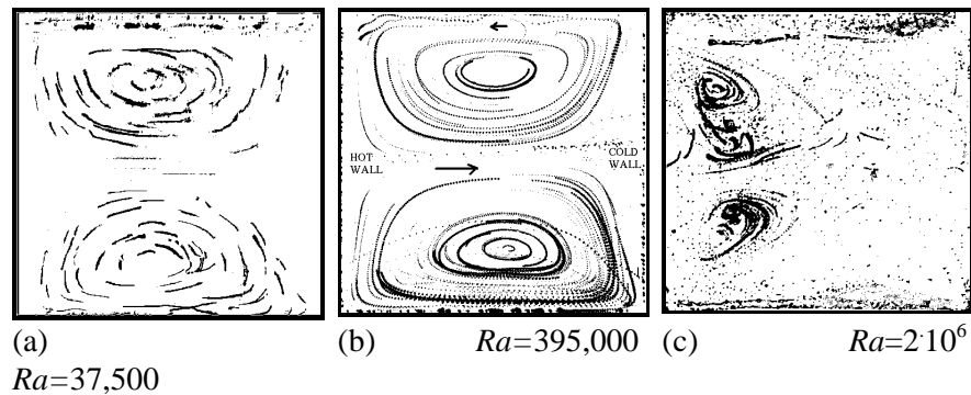
Figure 2. Steady state free surface flow pattern ( y=0.9 ); (a) - 24 superimposed images taken every 20s, (b) - 100 images taken every 20s, (c) - 25 images taken every 20s.
