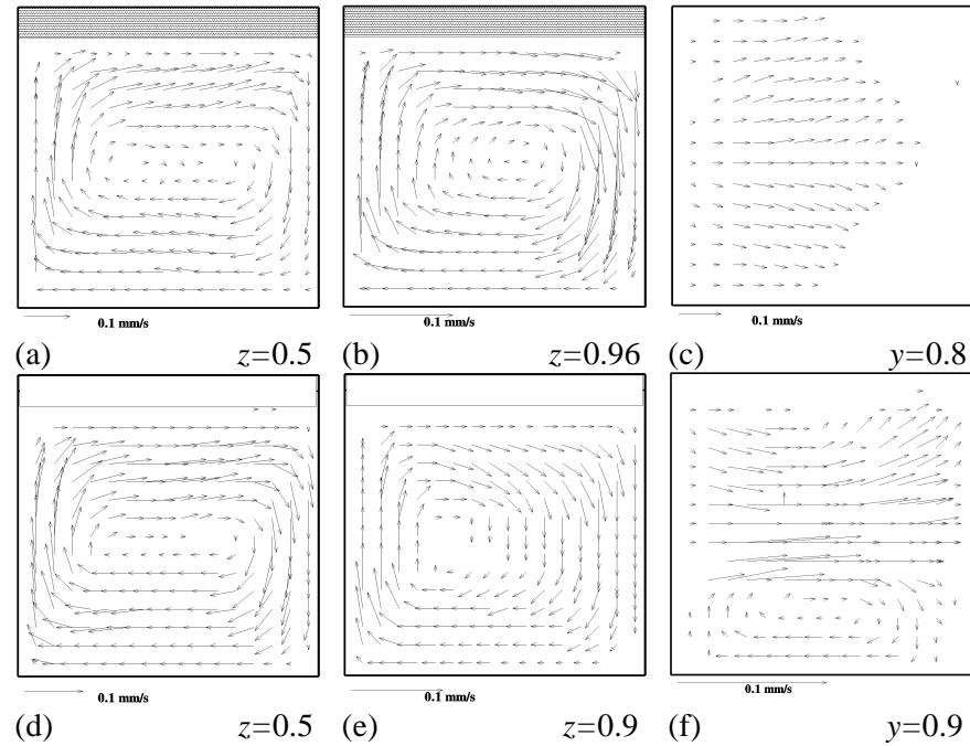
Figure 1. PIV measured velocity field at three cross-sections for closed cavity (upper row) and free surface case (bottom row); steady state; Ra=37,500 , Pr=8,700 .
