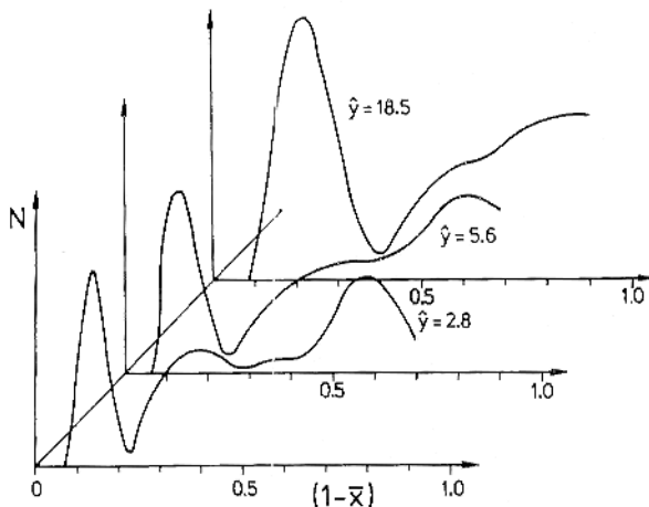
Fig. 5. Spatial droplet distribution for different distances from the channel inlet: \lambda = 15, Re = 1
