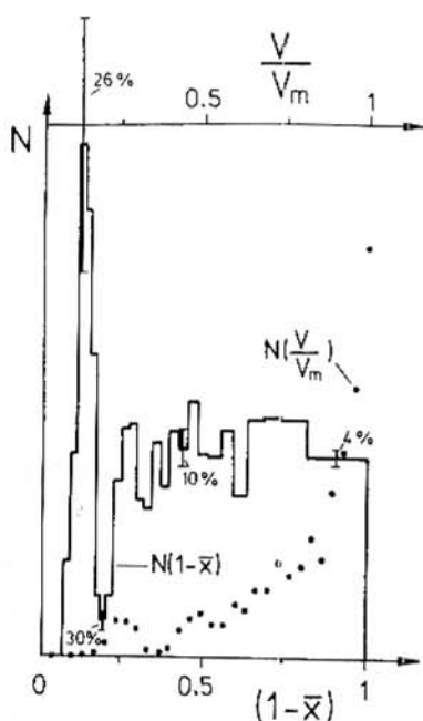
Fig. 2. Measured droplet velocity spectrum N\left(\frac{v}{v_m}\right) (dotted line) and calculated spatial droplet density distribution N(1-\bar{x}) (solid line): \lambda = 0.1 , \gamma = 10 mm, Re = 10^{-4}
