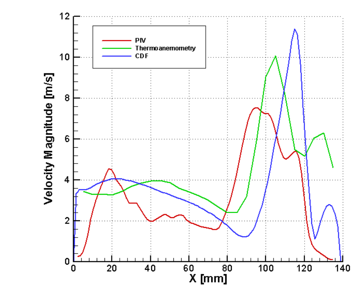
Measured and simulated velocity profiles along the centre line; configuration „A”
