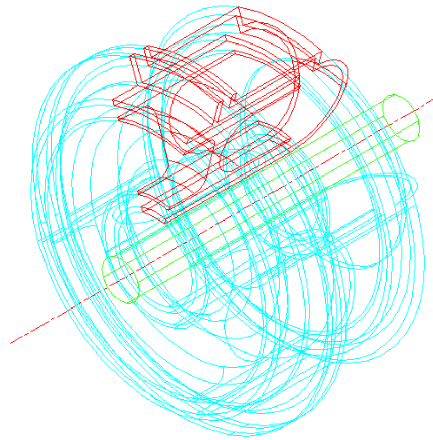
Selected sector of a gas turbine combustor
