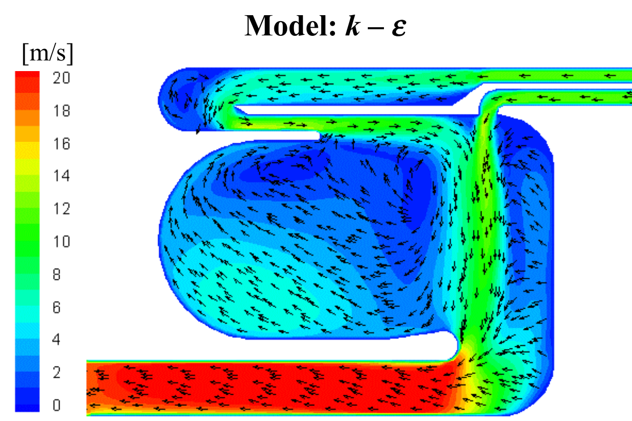
Configuration „A”: velocity vectors and contours of velocity magnitude
