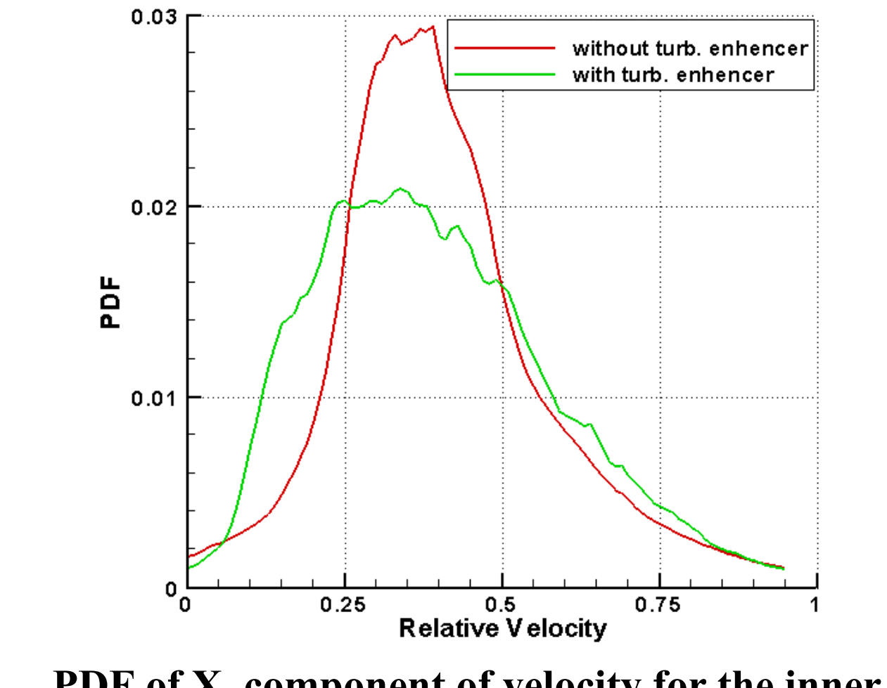
PDF of X-component of velocity for the inner vortex
