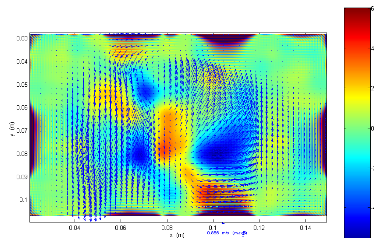
Filtered average velocity field and the vorticity contours with „turbulence enhancer”
