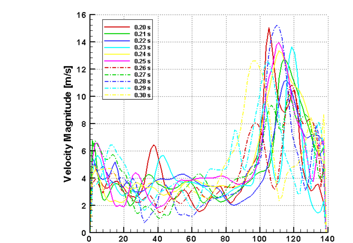
Velocity profiles for different time steps calculated by LES – model
