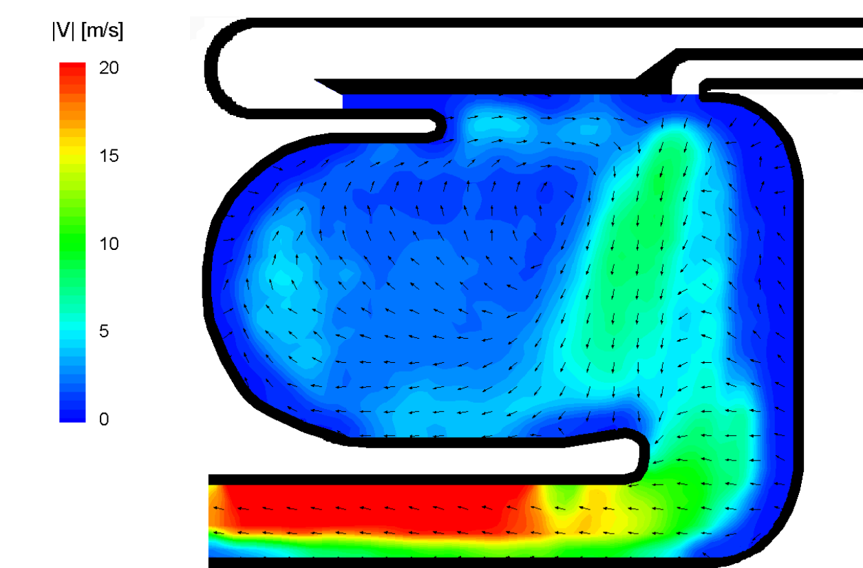
Configuration „A”: averaged velocity vectors and contours of velocity magnitude
