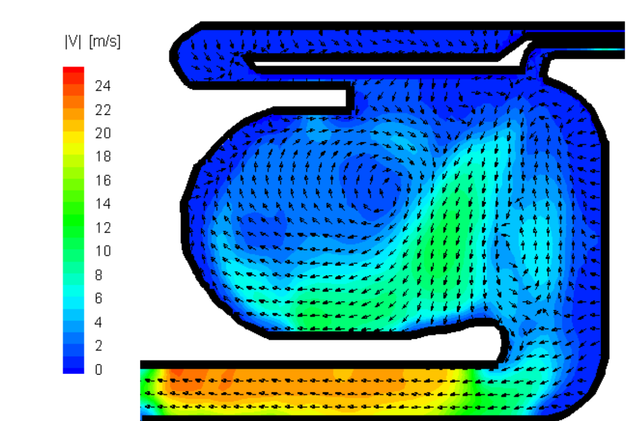
Configuration „C”: averaged velocity vectors and contours of velocity magnitude
