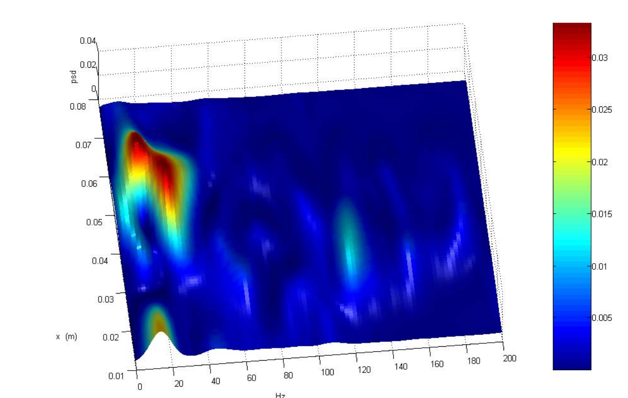
PSD of the Y-component of the velocity
