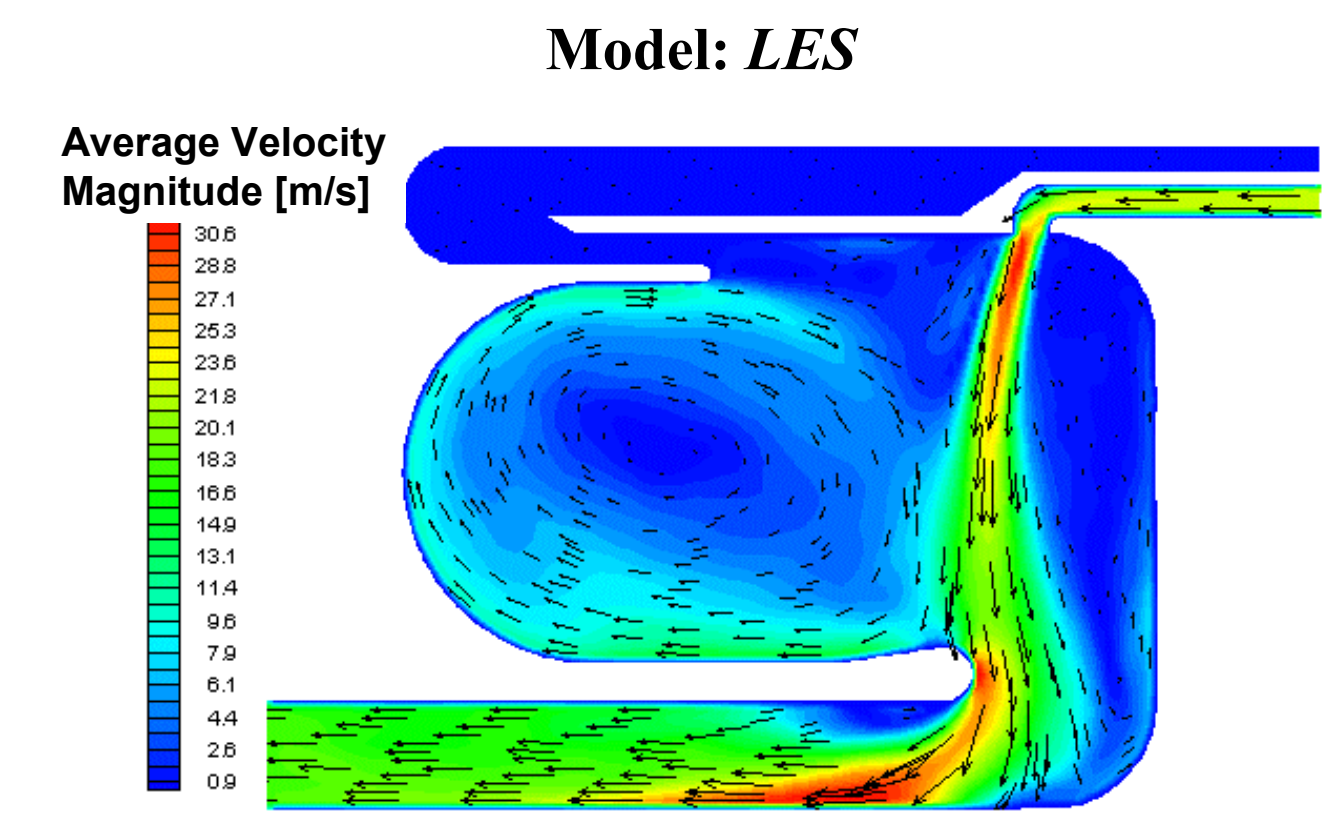
Configuration „C”: velocity vectors and contours of velocity magnitude
