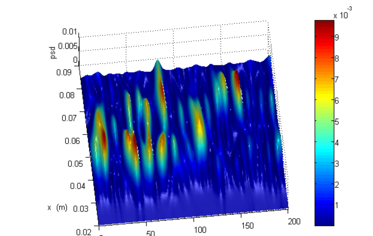
PSD of the Y-component of the velocity with „turbulence enhancer”
