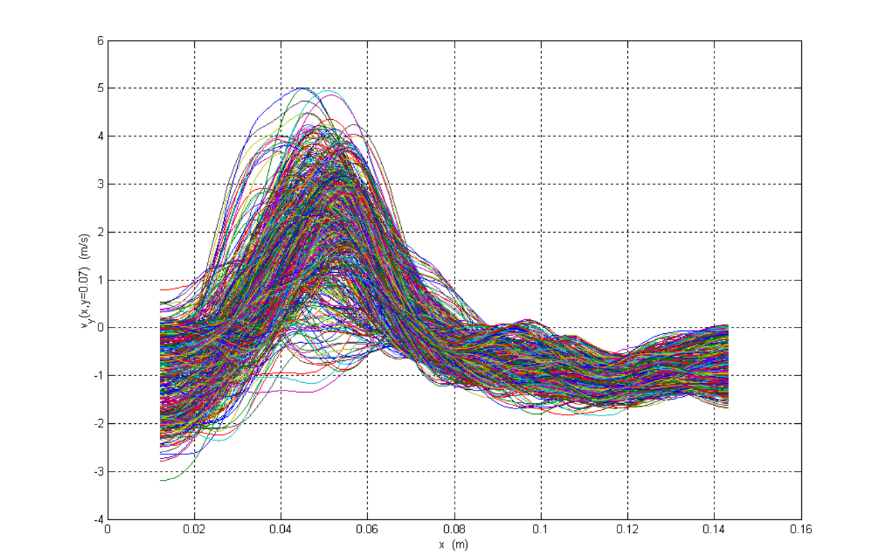
500 profiles of the Y-component of the velocity
