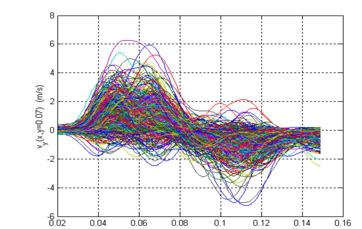
Profiles of the Y-component of the velocity with „turbulence enhancer”
