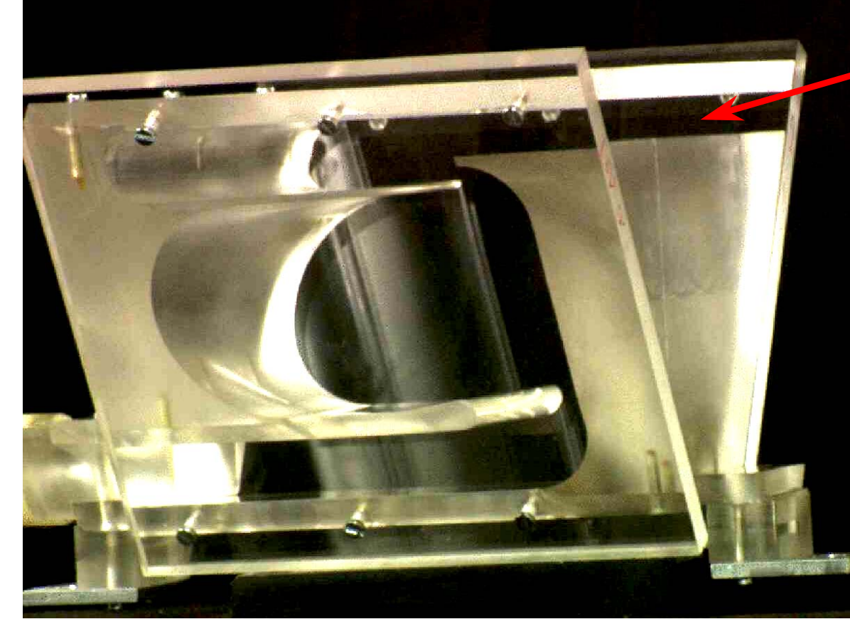
Plexiglas model of the combustor sector (60°)
