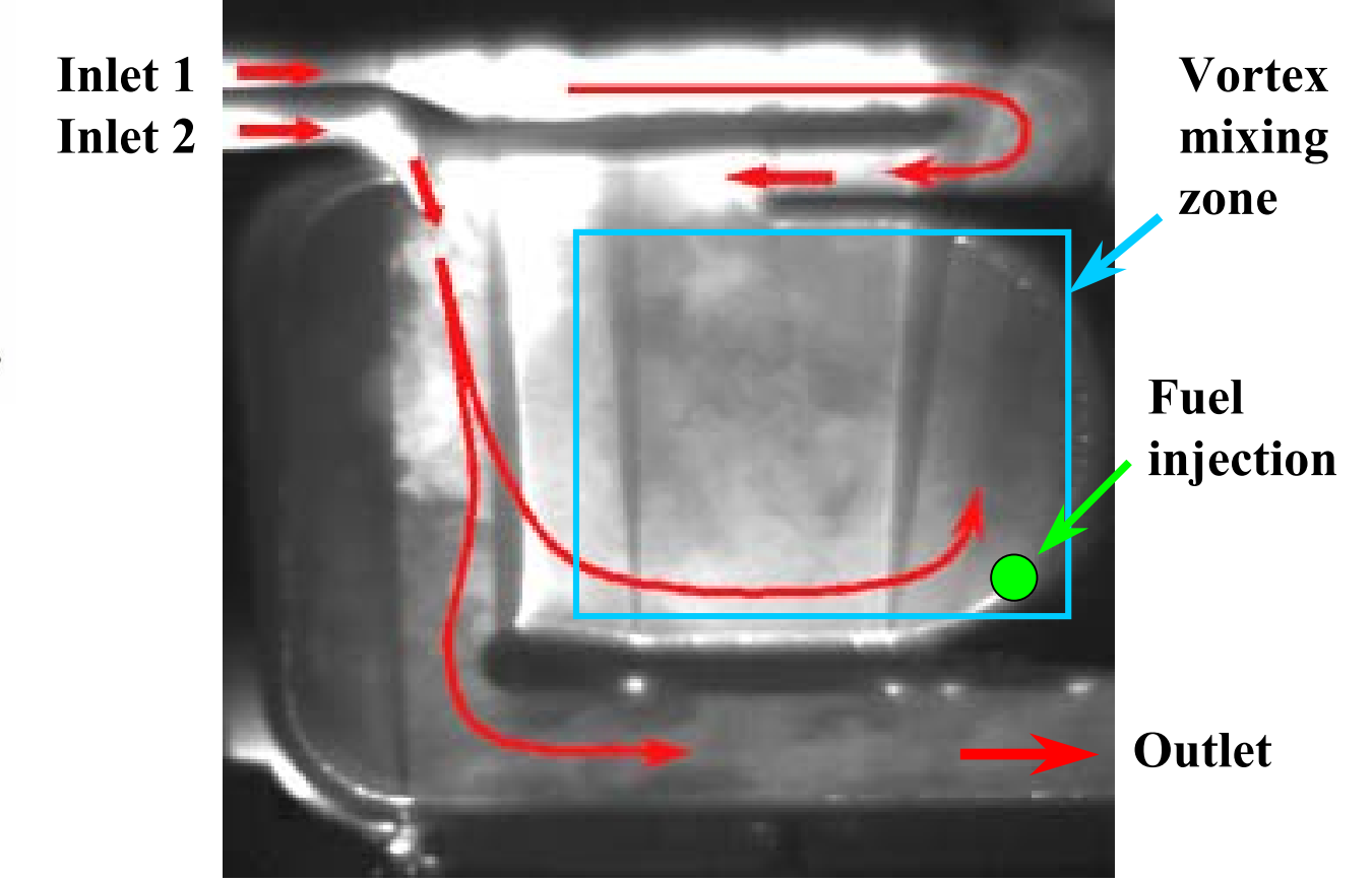
Flow visualization in the centre cross – section using high-speed camera
