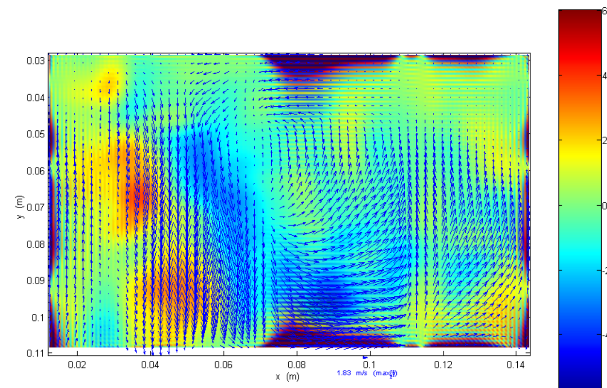
Filtered average velocity field and the vorticity contours
