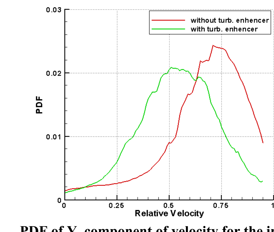
PDF of Y-component of velocity for the inner vortex
