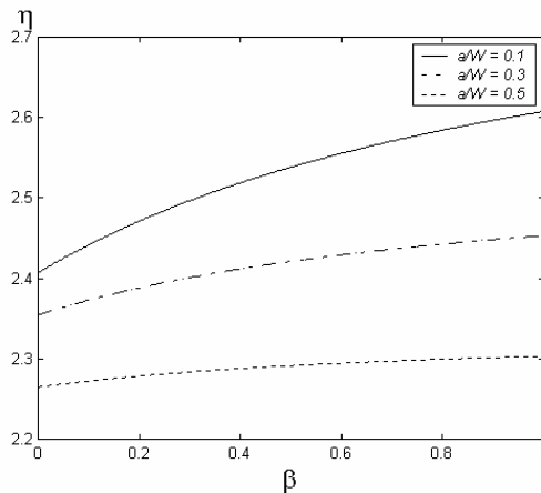
Figure2: \eta factor as a function of hardening coefficient \beta .
