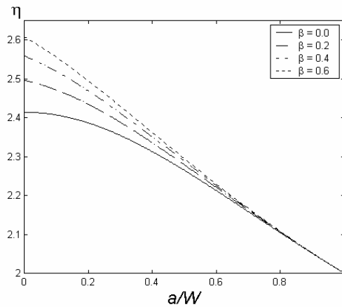
Figure3: \eta as a function of normalized crack length a/W .
