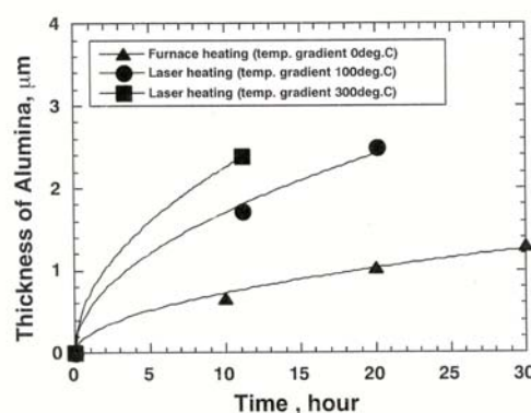
Fig.5 The effect of temperature gradient on the thickness of thermal growth oxidation, i.e., alumina
