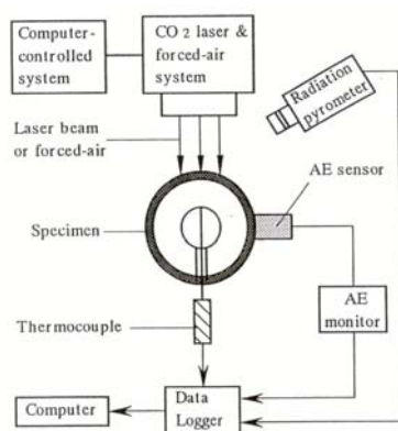
Fig.4 Schematic of the experimental setup for CO 2 laser heating method
