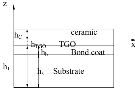
Fig.1 Crossing-section of thermal barrier ceramic coating system
