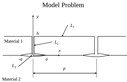
Figure 1. Initiation and growth of Interface cracks.
