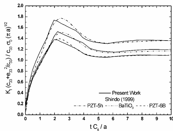
Figure 4. Mode I SIF versus dimensionless time for a Griffith crack under the action of normal impact loading
