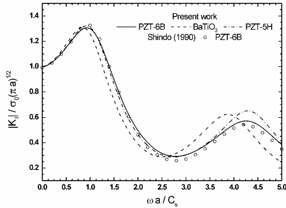
Figure 3. Mode I SIF versus dimensionless frequency for a Griffith crack under a plane harmonic wave
