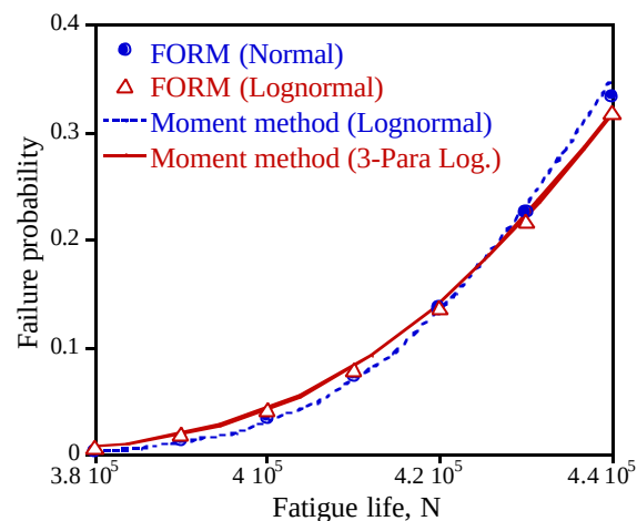
Fig. 2. Failure probability
