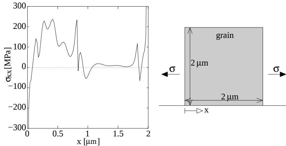
Figure 3. Stress profile at the free surface of a 2 \times 2 \mu\text{m} grain after 1897 cycles.
