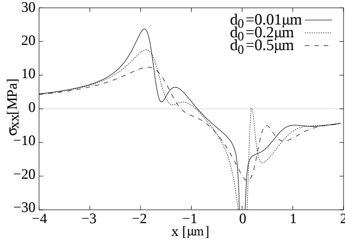
Figure 2. Stress profile at the free surface for different spacings of the first dislocation to the free surface.
