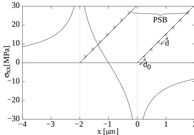
Figure 1. Idealized dislocation distribution in a PSB according to Brown and Ogin [1] and logarithmic singularity in the stress component \sigma_{xx} parallel to the surface at the root of the PSB.
