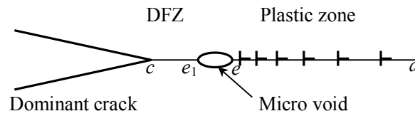
Figure .2 Schematic illustration of the coupling effect between fatigue and creep.
