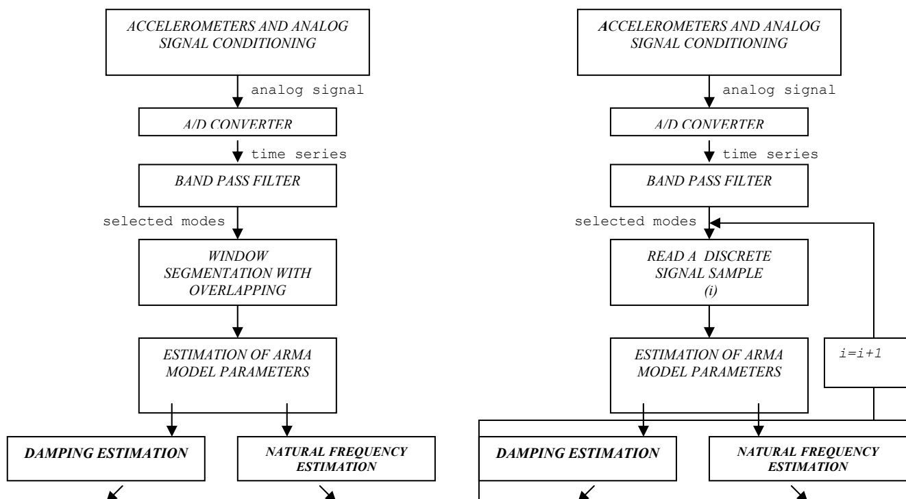
Figure 1. Schemes of formulated real time modal analysis a) signal segmentation based algorithm, b) model updating algorithm.
