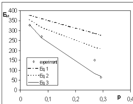
Fig. 1. Experimental values of elastic modulus vs. theory
