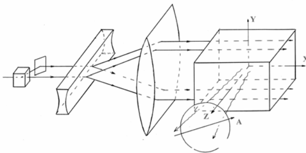
Fig.1. Schematic of optical slicing method.
