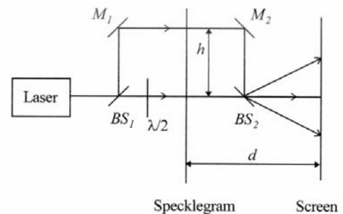
Fig.2. Schematic of the optical pointwise filtering method
