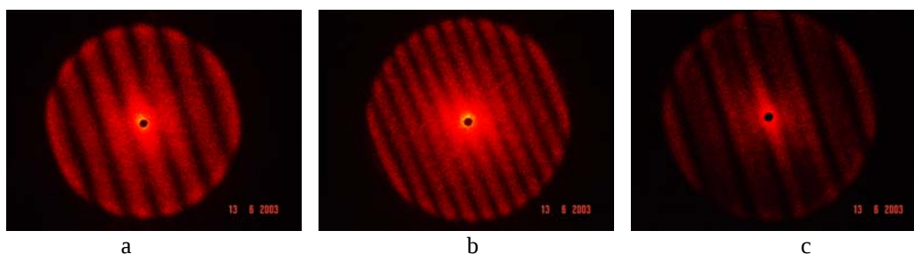
Fig.6. Young's fringe patterns (a, b) and moiré pattern (c).
