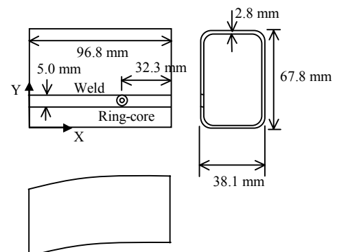
Fig. 2 Plan, elevation and side views of the hydroformed frame part
