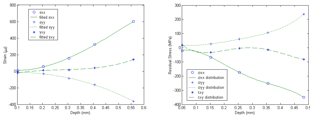
Fig. 3 Relieved strains and residual stresses on the laser weld
