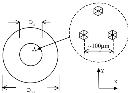
Fig.1 Schematic diagram of ring-core and ISSR
