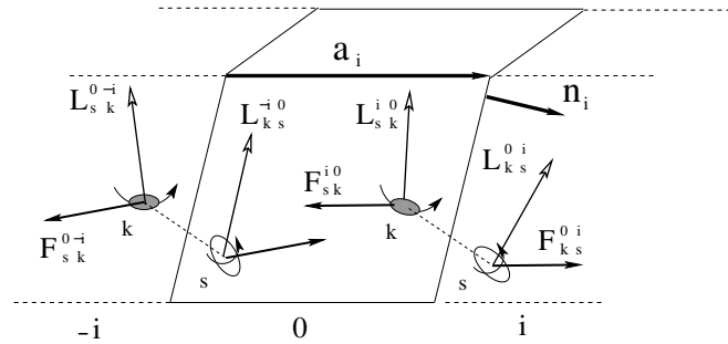
Figure 2. A cell of a crystal. Discrete model
