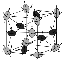
Figure 1. 1/8 of a cell of the Yttrium-Iron Garnet. Distribution of Fe.
