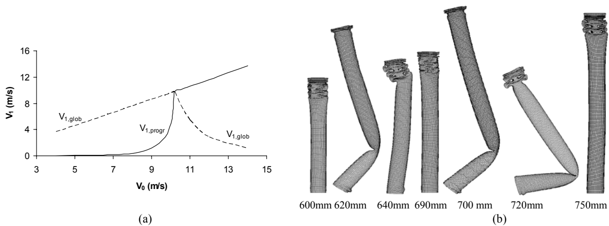
Figure 1 (a) Velocities V_1(t^*) at the end of the compressive phase: — progressive buckling mode, ---- global bending mode, L = 550 mm, h = 2.19 mm; (b) Buckling shapes of tubes made of an aluminium alloy, V_0 = 10.4 m/s and G = 209 kg.
