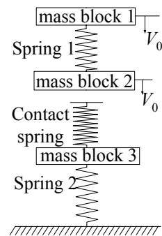
Fig. 3 A simple mass-spring collision system
