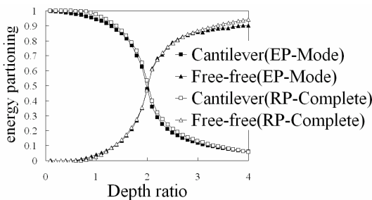
Fig. 1 Energy partitioning between two beams
