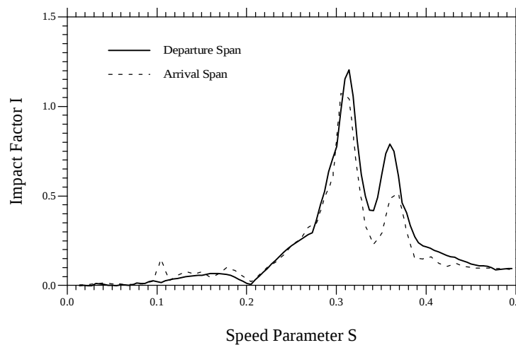
Fig. 2 Impact response of continuous truss bridge.
