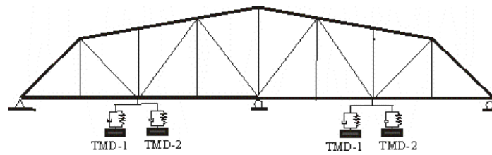
Fig. 3 Continuous truss bridge model with hybrid TMD systems
