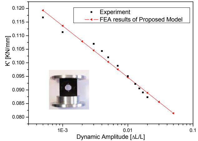
Fig 2 Comparison the experiment results with the FEA results of proposed model for complex shape test
