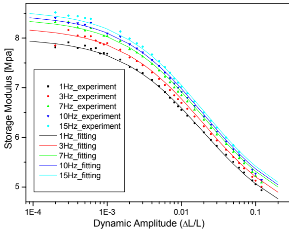
Fig 1 Curve fitting of tension test results
