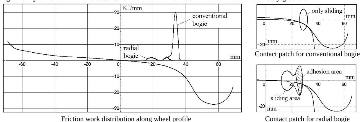
Figure 3. Results of railway simulation in even curve.
