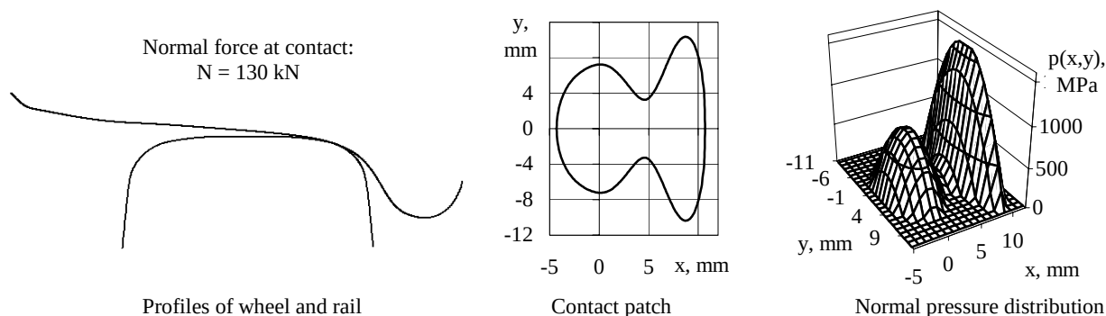
Figure 1. Example of normal contact problem solution.
