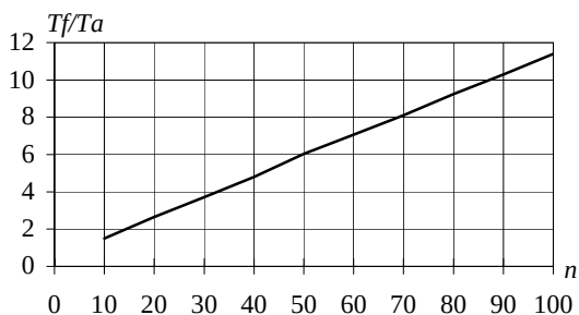
Figure 2. Ratio of required solution time of FASTSIM to time of analytical method.
