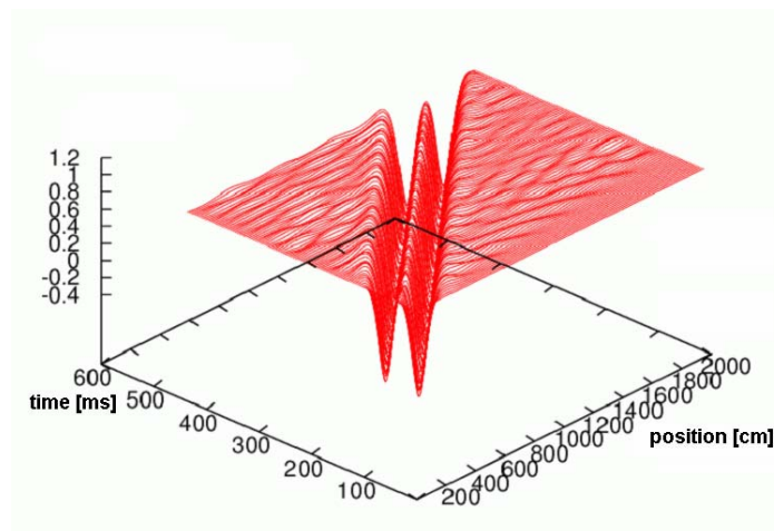
Fig. 4. Vertical displacements of a track obtained in the time-space domain.
