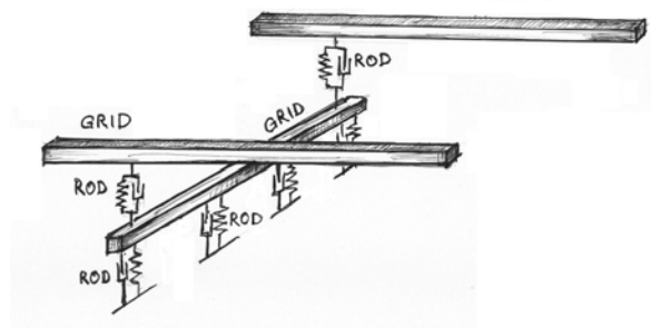
Fig. 3. Model of the track used in computational analysis
