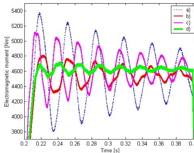
Figure 1. Electromagnetic moment of a driving motor with control unit versus time. Results of calculations for an electromechanical model: a) with preliminary selected settings of a control unit, b) after optimization of settings of a control unit, c) with a control unit before optimization and optimized some parameters of mechanical part, d) optimized control unit and parameters of a mechanical part
