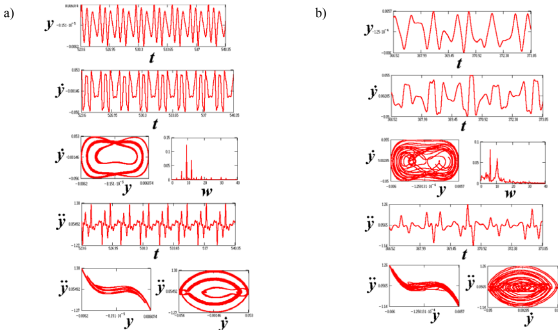
Figure 2. Time characteristics and phase trajectories of the system under consideration ( m = 3 ; \varepsilon = 0.5 \text{ s}^{-1} ; \alpha = 408 \text{ s}^{-2} ; \beta = 7660000 \text{ m}^{-2} \text{ s}^{-2} ; F_1 = 0.15 \text{ ms}^{-2} ; F_l = 0.075 \text{ ms}^{-2} ): a) combinative oscillations; b) chaotic oscillations.
