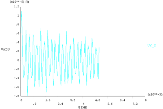
Fig 2: chuck vibration amplitude due to shock force (FEA)
