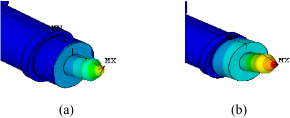
Fig 3: Displacement contour a) in acting force b) Free vibration
