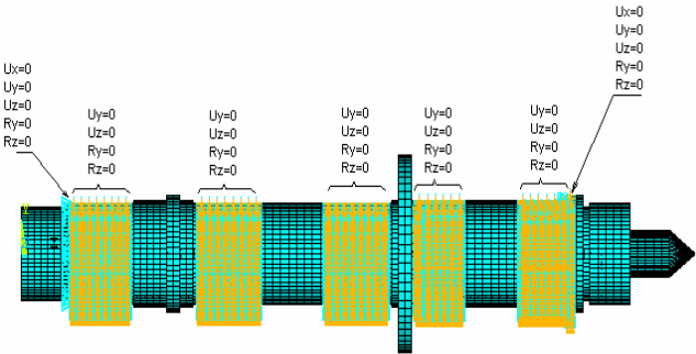
Fig 1: Applied boundary conditions on conventional spindle (Five bearing sets)
