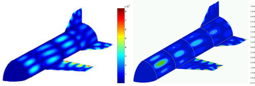
Figure 1: Comparison between the VTCR (left, 672 dofs) and NASTRAN (right, 28,800 dofs). The scales are the same
