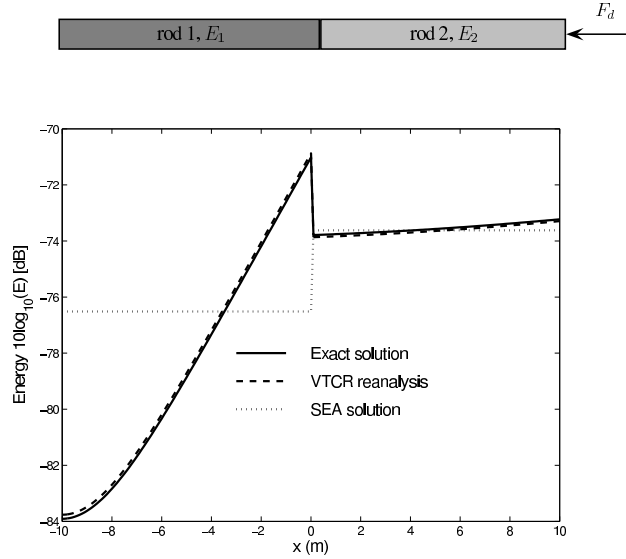
Figure 2: Reanalysis method applied to a rod problem
