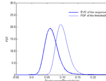
Fig.3 The EVD and the PDF of the threshold
