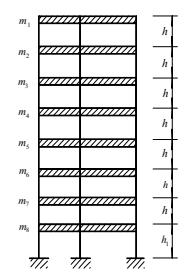
Fig.1 The 8-story frame
