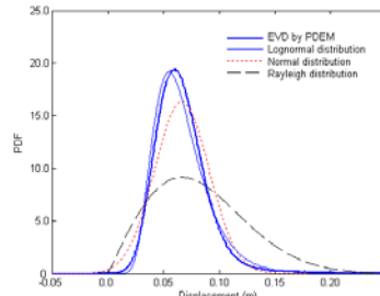
Fig.2 The EVD and widely used distributions
