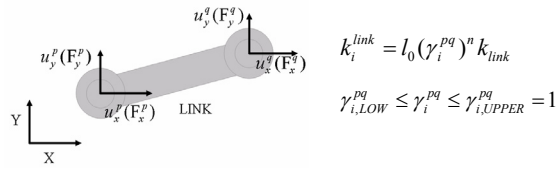
Fig. 3 Link element connecting nodes p and q at connection i . It has the design variable \gamma_i^{pq} .
