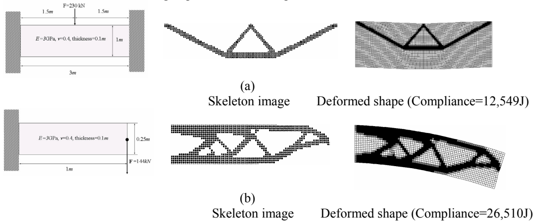
Fig. 4 A compliance minimization of geometrically nonlinear structures. (a) Mass constraint ratio=10%, 120 \times 40 4-node bilinear finite elements used, (b) mass constraint ratio=50%, 80 \times 20 4-node bilinear finite elements used.
