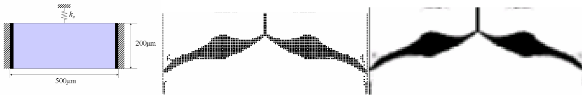
Fig. 5 Design of an electro-thermal-compliant actuator. Output displacement: 6.96 \mu\text{m} ( k_s = 100\text{N/m} , Mass constraint = 30%, Young's Modulus = 200 GPa, Poisson ratio = 0.31, thickness = 15 \mu\text{m} , the electric conductivity = 6.4 \times 10^6 \text{K}(\Omega\text{m})^{-1} , the thermal conductivity = 90.7 \text{W/(Km)} , the convection coefficient = 18.7 \times 10^3 \text{W/(m}^2\text{K)} , thermal expansion coefficient = 15 \times 10^{-6} \text{K}^{-1} , applied voltage = 0.3 volt).
