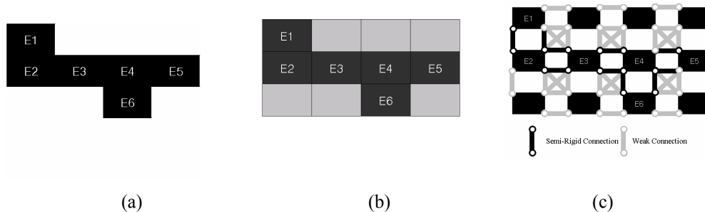
Fig. 2 Structural layout modeling. (a) A typical structural layout, (b) modeling by the standard element density method (Grey: Weak elastic elements, Black : Solid elements), (c) the modeling by the ECP method (Black Line : Semi-Rigid Connection: Grey Line : Weak Connection).
