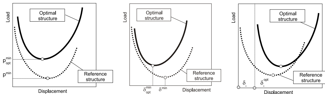
Figure 1. Maximization of lower critical loading when upper critical load is absent (left). Minimization of generalized displacement for lower critical load (middle). Maximization of generalized displacement for which unstable equilibrium begins (right).
