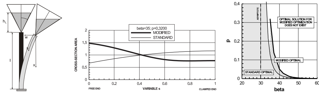
Figure 2. A column loaded by an attached vessel containing liquid (left). Standard and modified optimal column (middle). The three ranges for structural parameters (right).
