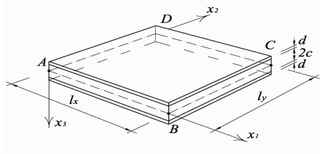
Fig.1 Sandwich plate
