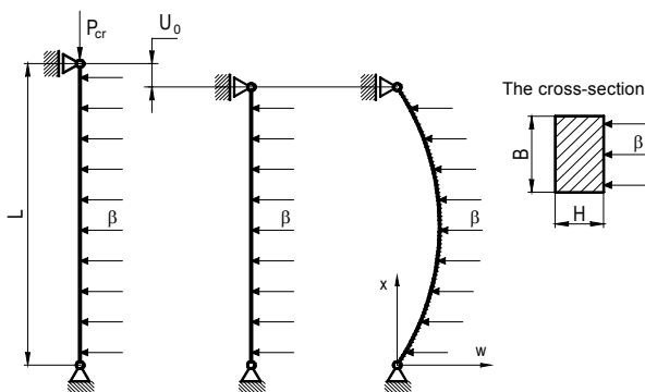
Figure 1. Column with chosen supports, under loadings controlled by displacement U_0 or force P_{cr}
