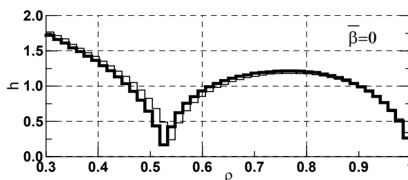
Figure 4. Distribution of dimensionless thickness h(\rho) of annular plate with immovably clumped inner edge, movably simply supported and loaded outer edge.
