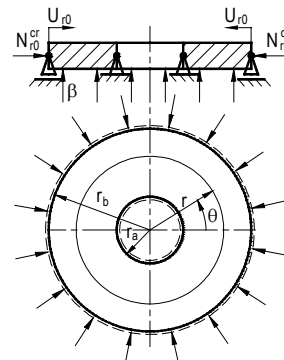
Figure 2. Annular plate with chosen supports, under loadings controlled by displacement U_{r0} or force N_{r0}^{cr}
