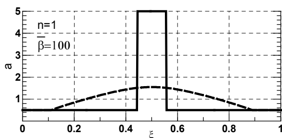
Figure 3. Distribution of dimensionless cross-sectional area a(\xi) of simply supported column on an elastic foundation
