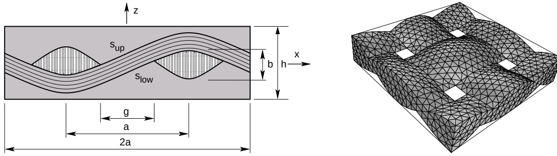
Figure 1. Idealized Periodic Unit Cell, (a) Geometrical model, (b) Example of finite element mesh
