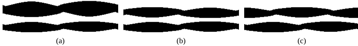
Figure 2. Artificial bitmaps of mesoscale geometry with typical tow misalignments, (a) different layer heights (PUC #1), (b) layers shifted by a (PUC #2), (c) layers shifted by a/2 (PUC #3)
