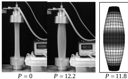
Figure 1 – Sequence of equilibrium configurations. Membrane under constant traction ( \Delta L/L=1 ) and increasing air pressure and FE results. P(10^{-4} \text{ MPa}) .
