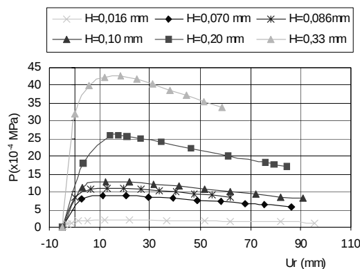
Figure 3 – Influence of the membrane thickness on the load-displacement response. Limit point instability
