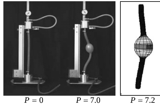
Figure 2 – Sequence of equilibrium configurations. Unstressed shell under increasing air pressure and FE results. P(10^{-2} \text{ MPa}) .
