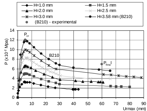
Figure 4 – Influence of the shell thickness on the load-displacement response. Limit point instability
