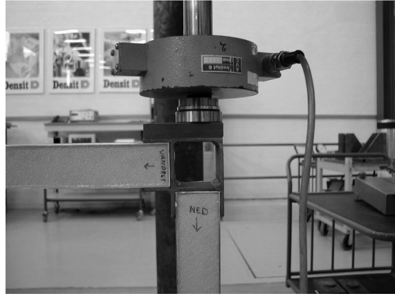
(b) Joint and loading device.
