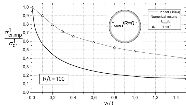
Fig. 4 Imperfection-sensitivity of the imperfect partially filled shell compared to the imperfection-sensitivity of the unfilled shell
