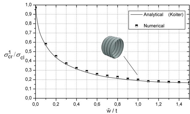
Fig. 2 Imperfection sensitivity of the unfilled shell. Analytical vs. numerical results
