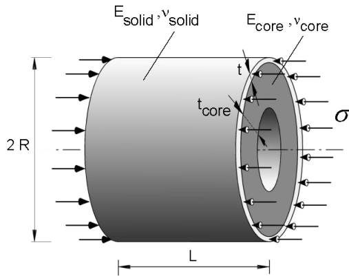
Fig. 1 Shell and load configuration
