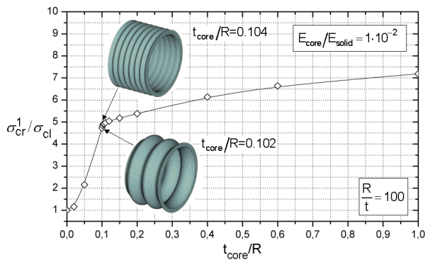
Fig. 3 Influence of the core-thickness on the bifurcation stress of the perfect configuration (relative to the classical buckling stress of the unfilled cylindrical shell)
