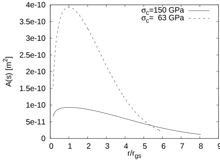
Figure 2. For two strings in the radial relative equilibrium configuration on the geostationary orbit around the Earth the areas of their cross-sections for carbon nanotubes with different admissible tensile stresses \sigma_c are given. The curve denoted by \sigma_c = 150 GPa corresponds to nanotubes of theoretical maximum strength resulting in a strain of \epsilon = 0.238 , whereas the curve denoted by \sigma_c = 63 GPa corresponds to nanotubes of the strength measured experimentally in [7]. The corresponding strain is \epsilon = 0.1 . For both strings the calculations have been performed with endmasses of 1 kg. Moreover the ratio between the cross-sectional area at the geostationary height to the area at the surface of the Earth follows from the figure to 1.41 for \sigma_c = 150 GPa and 2.50 for \sigma_c = 63 GPa.
