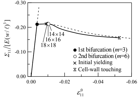
Fig. 3. Macroscopic stress-strain relation under equi-biaxial compression.
