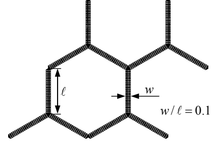
Fig. 1. Subunit of hexagonal honeycomb.
