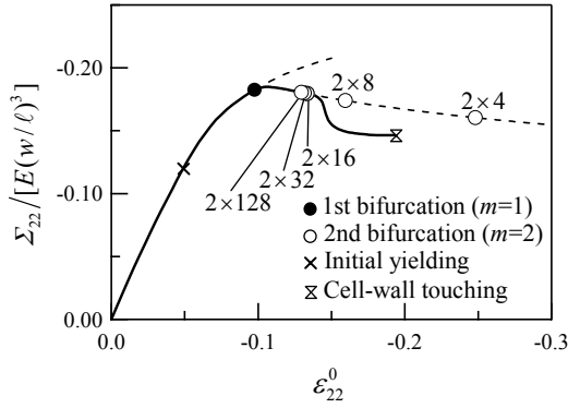
Fig. 2. Macroscopic stress-strain relation under uniaxial compression.
