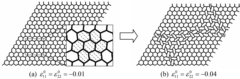
Fig. 4. Change in deformation of Y_{16 \times 16} due to the second bifurcation under equi-biaxial compression.
