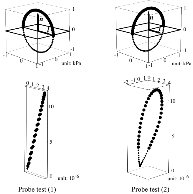
Figure 2. Plastic strain increment
