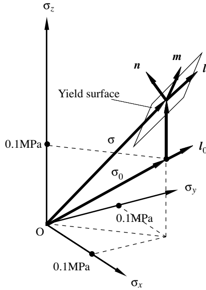
Figure 1. Loading path
