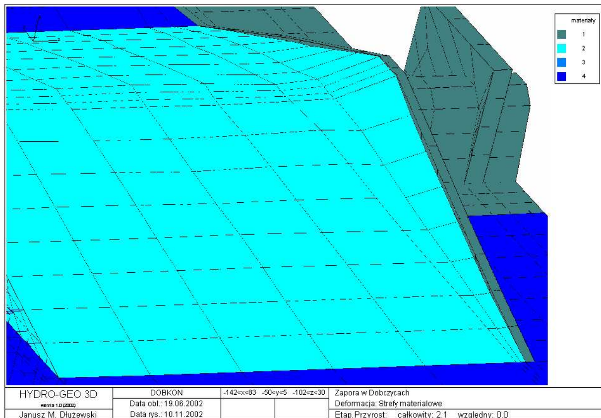
Figure 3 Slide on the surface of contact between the retaining wall and earth dam
