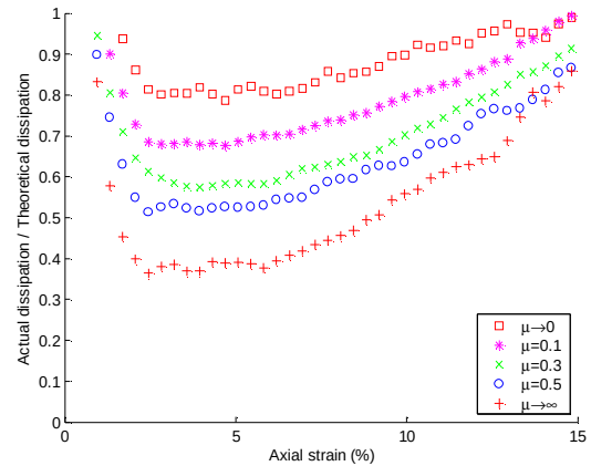
Figure 2. Comparison of dissipation-rate functions.
