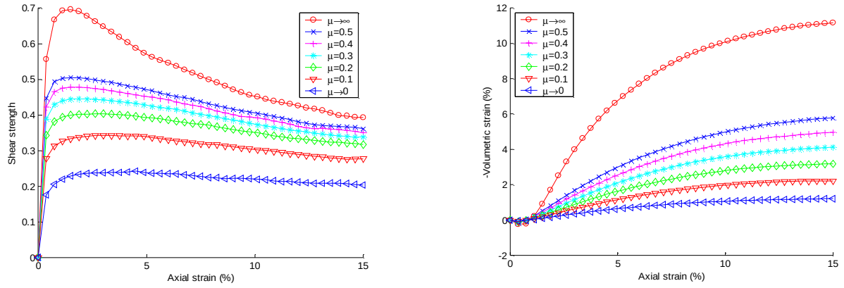
Figure 1. Macroscopic behaviour as a function of imposed axial strain for various interparticle friction coefficients \mu .
