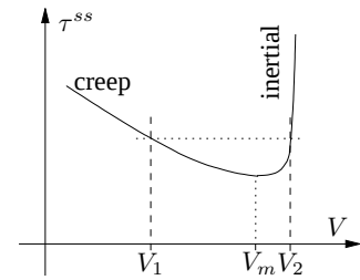
Figure 1. Dry friction law (cf. [1])
