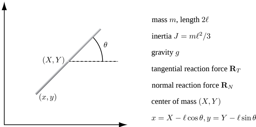
Figure 1. The mechanical set-up.
