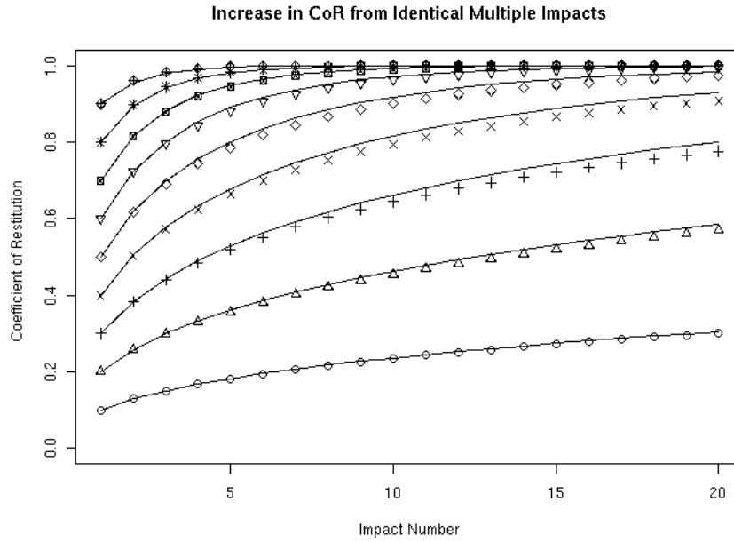
Figure 2. Discrete symbols denote the corresponding solutions to (1), for initial values C_1 between 0.1 and 0.9 in steps of 0.1, as a function of the number of impacts. The continuous lines in Figure 2 are the curves described by (3).
