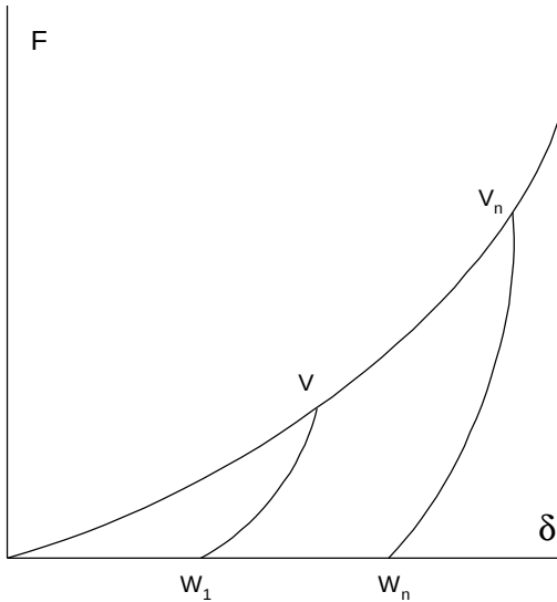
Figure 1. Sketch of the typical force-displacement curve for repeated, identical, quasi-static impacts between two elasto-plastic bodies. The steep path along the w entries is assumed to be wholly elastic, while the upper curve along the v entries is assumed to be essentially fully plastic.
