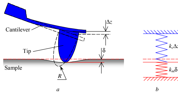
Fig. 1. Schematic diagram of the interaction between probe and sample surface (a) and mechanical model of the tip-sample interaction (b)
