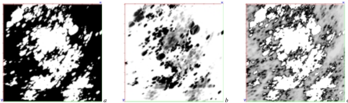
Fig. 2. Visualized results of simulation of contact between two rough DLC surfaces: a – real contact area, b – distribution of contact pressure, c – molecular adhesive forces between the surfaces
