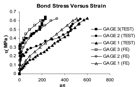
Figure 2- Bond stress vs. strain graph for different gages along the embedment.
