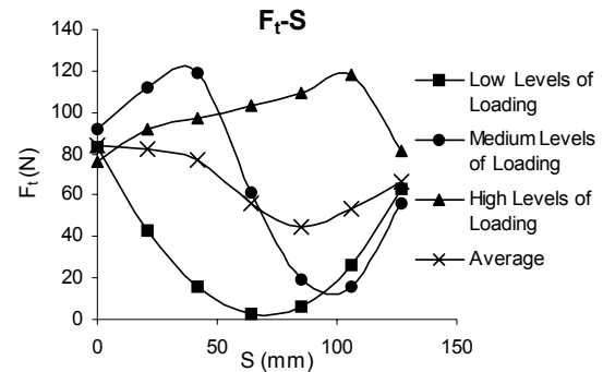
Figure 5- Variation of F_t along the embedment.
