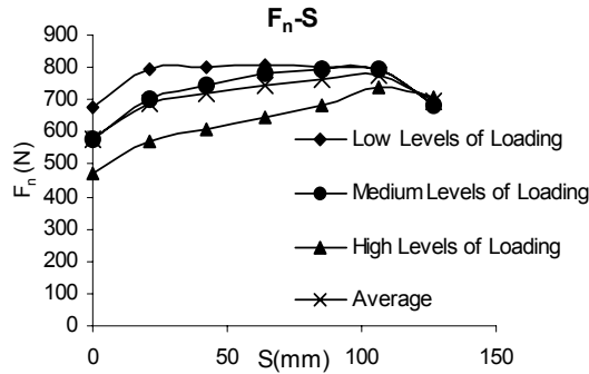
Figure 4- Variation of F_n along the embedment.
