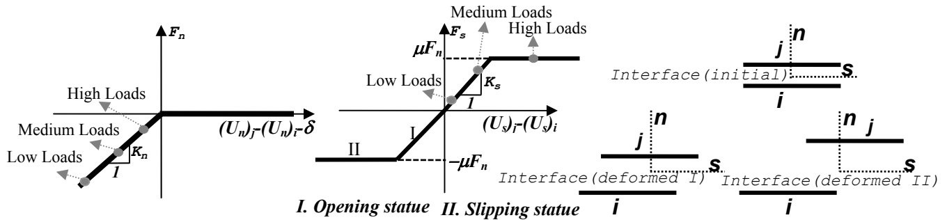
Figure 3- Normal and tangential mechanical behaviour along the boundary.
