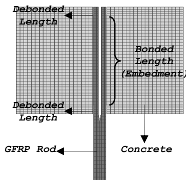
Figure 1- Typical shape of the axisymmetric FE model.
