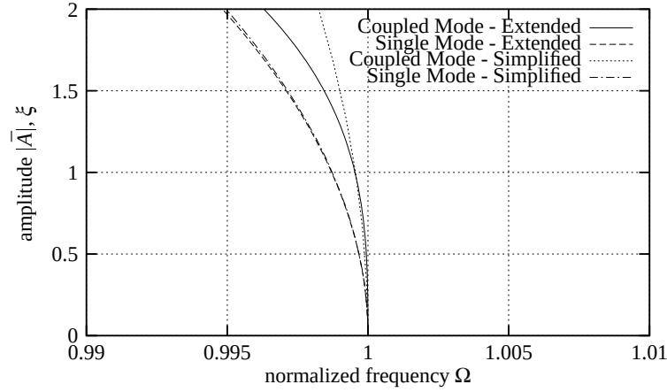
Figure 1. Amplitude-frequency curves for Single Mode and Coupled Mode nonlinear vibrations of isotropic shell. Comparison between Simplified Analysis (vibration mode amplitude |A| ) and present Extended Analysis (vibration mode amplitude \xi ); \Omega = \omega/\omega_{01} .
