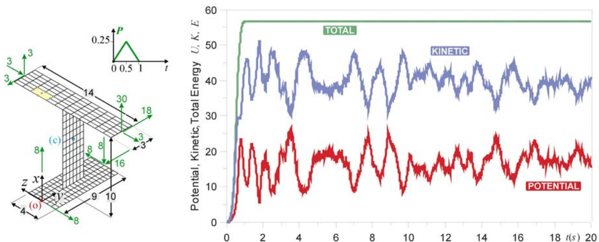
Fig. 2 Three intersecting plates. Geometry and energy functions
