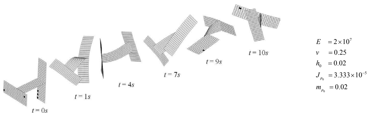
Fig. 3 Three intersecting plates. Data and shell deformations
