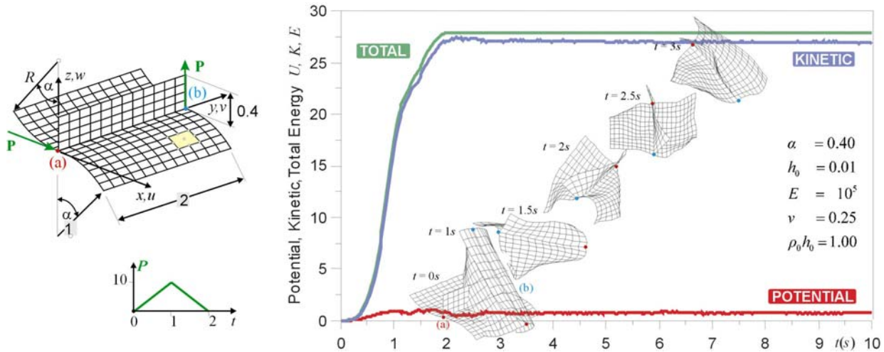
Fig. 1 Cylindrical panel. Geometry, energy functions and shell deformations
