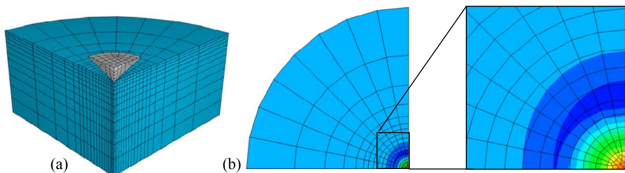
Figure 1: Finite element model of indentation test (a) and contours of the imprint mapping (b).
