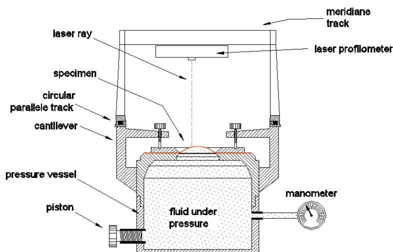
Figure 2: Schematic representation of the membranometer.
