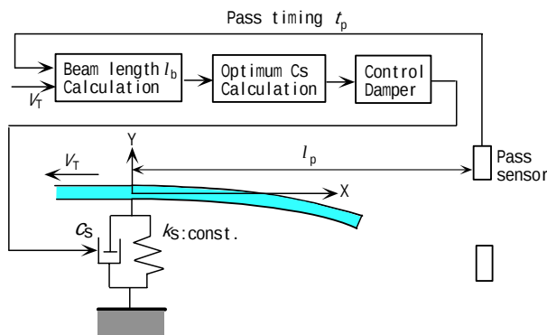
Fig.1 Planar beam model moving along the axial direction using FEM formulation
