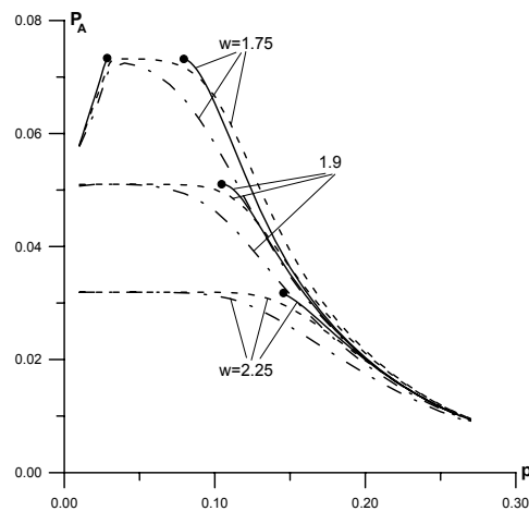
Fig. 1. Amplitude-frequency curves for nonlinear forces in a single gear transmission.
