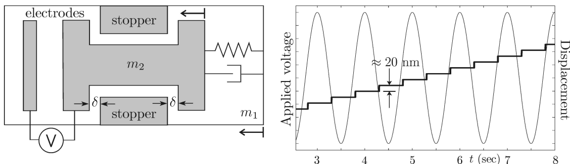
Figure 1. Schematic of microactuator (left panel) and displacement pattern resulting from a periodic voltage excitation (right panel).
