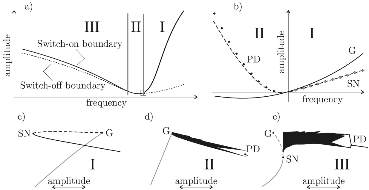
Figure 2. Transition scenarios between non-impacting to impacting asymptotic dynamics under variations in driving amplitude and frequency (G=grazing contact, SN=saddle-node bifurcation, PD=period-doubling bifurcation). In a), the solid line corresponds to the onset of impacting motion under increases in amplitude, while the dashed line corresponds to the termination of impacting motions under decreases in amplitude. Panel b) shows a blow-up of the rectangular region in a) at the boundary between Type I and Type II transitions illustrating the close agreement between the analytical theory (curves) using discontinuity mappings and numerical data (circles and squares). Panels c), d), and e) exhibit the bifurcation scenarios associated with the switching between impacting motions (black) and non-impacting motions (gray) that occurs under variations in driving amplitude. Here, solid curves correspond to stable periodic motions and dashed curves to unstable periodic motions. The black regions correspond to impacting chaotic attractors.
